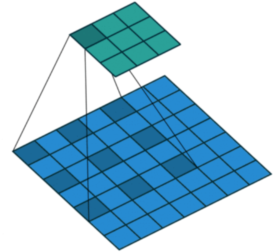
2-dilated convolution
